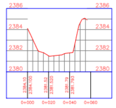
X-X2 PROFILE
