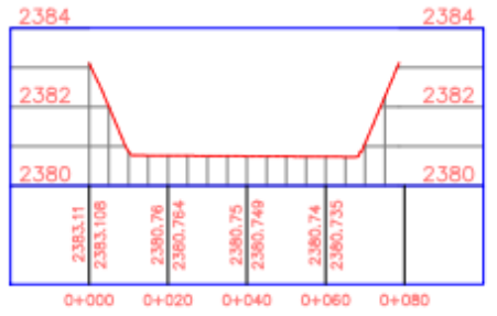
X-X PROFILE
